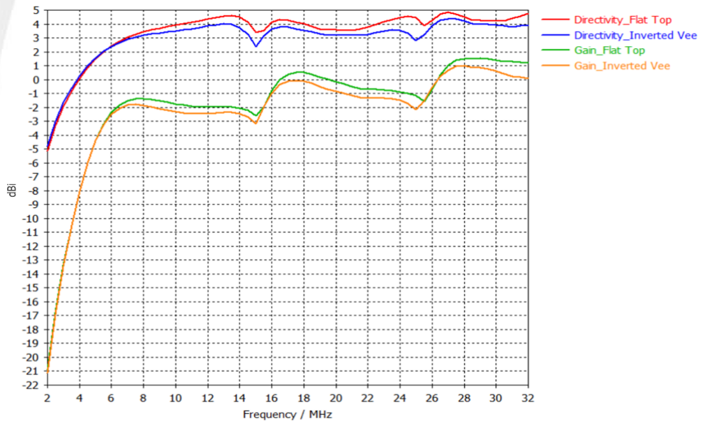
Inverted Vee and Flat Top Folded Dipole Antenna's Directivity and Gain
