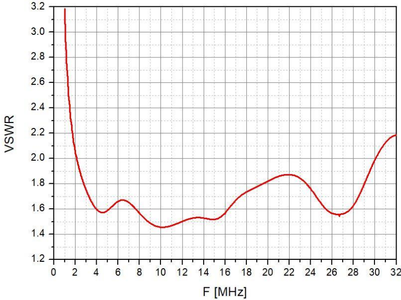
VSWR of Flat Top Folded Dipole Antenna
